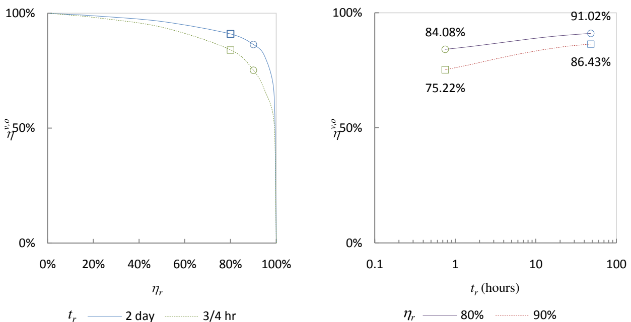
Figure 4: Difference in performance between a slow and fast resetting optimised first-flush device
